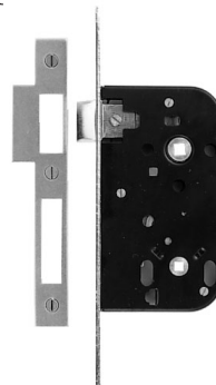
European Privacy Mortise Lock (Lever/Lever) No. 8401-02
