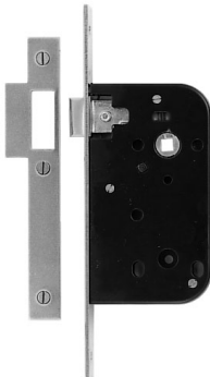
European Passage Mortise Lock (Lever/Lever) No. 8401-01
