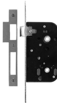
European Privacy Mortise Lock (Lever/Lever) No. 8401-03
